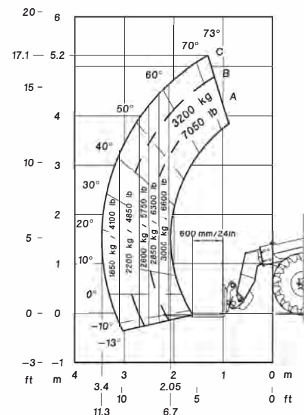
Load Chart - on tires with 48" forks compliant with ANSI/ITSDF B56.6
